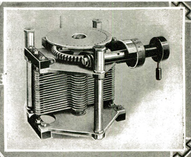
View Above Shows the Fine Workmanship on New American Built Precision Condenser. This Condenser is Suitable for All Kinds of Radio Work, and Particularly for High Class Receiving Sets and Various Radio Measurements. It is Provided With Two Finely Graduated Dials of the Highest Accuracy, and the Slightest Movements of the Rotary Plates can be Effected by Means of the Worm Wheel and Gear Shown, the Worm Being Turned by the Insulated Handle Shown at the Extreme Right.
