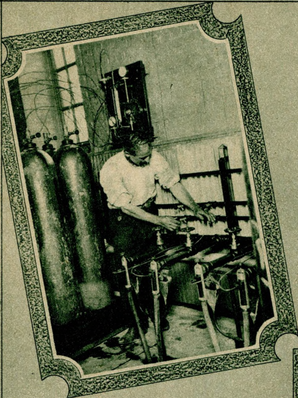
Applying Chlorine Gas at the Kensico Reservoir for Sterilizing the Water Supplied to New York City. The Gas is Received in Liquid Form Comprest in Cylinders. The Croton Supply is Treated Similarly and Smaller Plants in the Catskills and Croton Watersheds Treat the Streams Before Entering the Reservoirs.—(Copyright by Keystone.)
