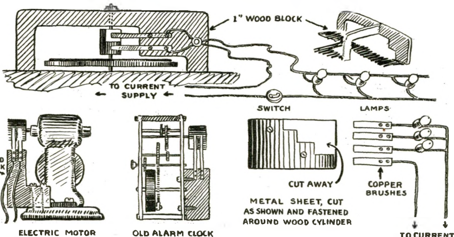
An Interrupter or Flasher for Christmas Tree Lights May Be Constructed in Several Ways, as Here Shown. It May Comprise a Segmental Drum, Rotated by a Phonograph Motor, by a Battery Motor, or Again by an Old Alarm Clock. Fig. 5.
