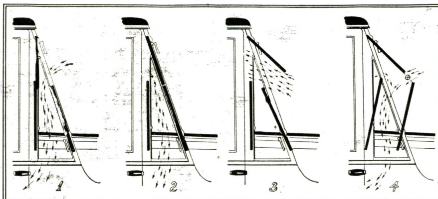
One of the Latest Innovations in Motor-cardom Is This Duplex Windshield, Which Can Be Made Storm-proof and Yet Provide Ample Ventilation, Simply by Manipulating the Component Parts of the Shield. The Arrows Show the Various Air Current Paths Which Can Be Provided at Will.
