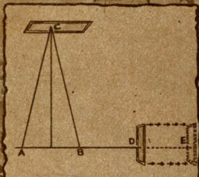
A POINT WHERE LIGHT ORIGINATED B POINT WHERE LIGHT REFLECTED FROM MIRROR 'C' IS RECEIVED D MIRROR IN FIRST POSITION MOVING TO 'E' BEFORE THE LIGHT FROM 'A' IS REFLECTED BACK TO 'B'
