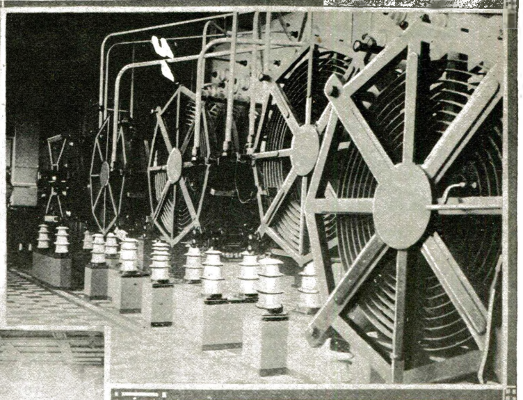
Upper Left-hand View Shows the High Frequency Dynamos in the Transmission Station at Nauen. It Will Be Noted How Carefully and Artistically the Apparatus Is Laid Out With Inlaid Rubber Floor Mats to Protect the Attachés From Shock When Touching the Machines While in Operation. In the Center of This View Can Be Seen a Centralized Switch for Directing the Energy From Each of the Dynamos to the Condenser and Other Power Rooms.
