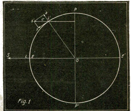
The Circle Represents the Section of the Earth With Axis PP' and Equator EE'. The Arrow SL Represents the Centrifugal Force at the Equator. Nearer the Pole S'L' Represents the Diminished Centrifugal Force and of This Only a Part, the Radial Component RL', Operates to Reduce the Weight of Any Object.
