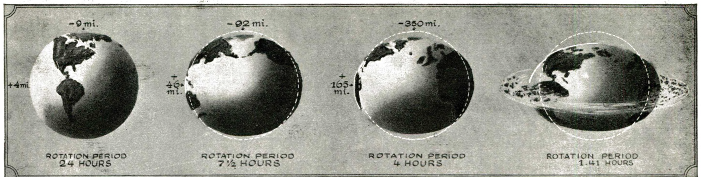
Our Earth Bulges About Four Miles at the Equator and Is Flattened About Nine Miles at the Poles, Due to the Rotational Speed of the Earth, Which at the Equator Is 1039 Miles An Hour. If the Earth Were Standing Still, the Globe No Doubt Would Have Been a Perfect Sphere. The Other Illustrations Show the Equatorial Bulge of the Earth and the Polar Flattening As the Earth Increases Its Rotational Speed. If It Were to Make a Complete Revolution In 1.41 Hours, the Bulge Would Become So Great That Objects Near the Equator Would Begin to Fly Off As Shown In the Last Picture, and As a Matter of Fact the Earth Would Begin to Break Up at Such a Tremendous Speed. Chances Are That the Earth Before It Had Cooled Revolved At a Different Speed Than It Does Now, But All Geological Data Point to the Fact That the Earth's Rotational Speed Has Neither Increased Nor Diminished Appreciably During the Ages.
