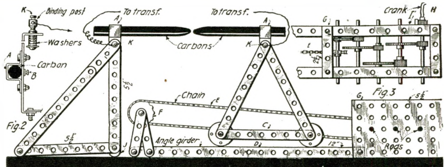
Fig 1 A Clever Experimental Arc Light Built From Meccano Toy Parts. The Arc Light Was Successfully Operated From a Toy Transformer on 26 Volts.
