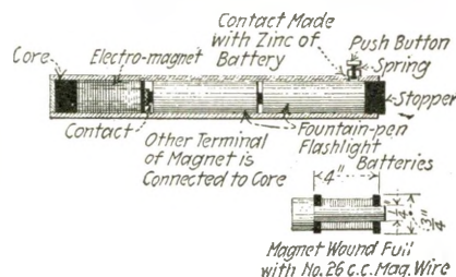
The Magic Wand Here Shown Can Be Built from an Old Electro-Magnet and a Fountain Pen Flashlight Battery.
