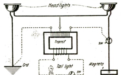
Wiring Diagram With Home-made Auto-transformer for Ford Headlights, Permitting One Lamp to Burn if the Other Goes Out.
