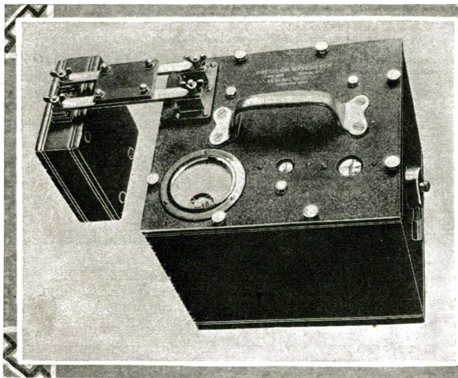
New Precision Wavemeter Designed for the Use of Students and Engineers Who Desire the Highest Accuracy in Making Various Wave-length, Inductance and Frequency Measurements. This Wavemeter Comprises a Very Accurate Plate Condenser as Well as an Inductance and a Thermo-galvanometer. No Buzzers or Other Paraphernalia are Included in the Circuits; Thus Providing an Instrument Having a Minimum of Leads and Permitting Their Resistance to be Made Negligibly Small. Range Is 75 to 24,000 Meters.
