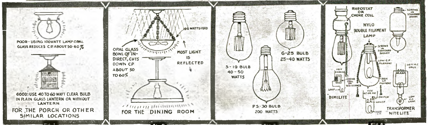
Some Practical Hints for Those Desiring the Highest Economy in Electric Lighting Are Shown in the Lower Illustrations, Figs. 1 to 4. Fig. 2 Shows How Approximately One-half the Candle Power Produced Is Utilized in Reflecting the Light Upward to the Ceiling and Back Again. Fig. 3 Shows the Three Principal Types of Incandescent Lamps, While Fig. 4 Shows the Three Leading Types of Nite-lights, Which Also Have Many Other Uses, of Course.
