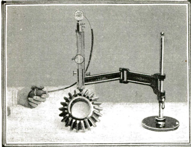
The Machine Shown Above Is Known as the "Scleroscope" and Is Used for Testing the Hardness of Steel or Other Metals by the Degree of Rebound of a Tiny Ball of Metal. This Ball Is Dropped from a Fixed Height to the Surface of the Metal. Rebounding Within a Glass Tube on Which Graduations Are Marked, the Reading Being Observed Thru a Magnifying Glass.
