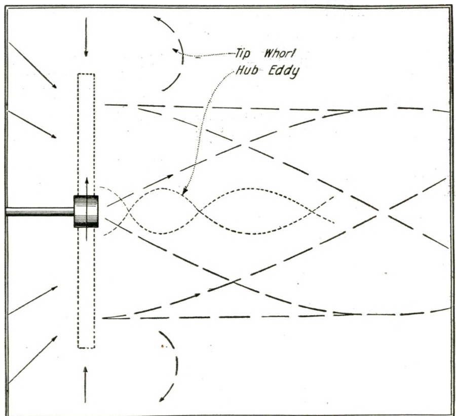
Analytic Diagram Showing Direction and Scope of Various Air Currents, Including the "Tip Whorl" and "Hub Eddy" for Rotating Propeller Blade. Much Can Be Gained by a Little Study of the Science of Air Propellers, Whether for Fan Blades or for Airplanes, as There Is Entirely Too Much Waste at the Present Time in Both of These Types of Propellers.
