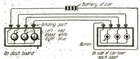
Simple Direction Indicator for Use on Motor Cars.
