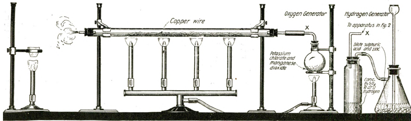
Fig. 1 Heating a Metal in the Air, the Metal Being Placed in a Crucible.
