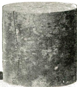
This Cylindrical Piece of Steel Burst at an Unexpected Moment and Nearly Killed a Tool-maker in the Great General Electric Works, Who Was Totally Unprepared for any Such Action as Here Occurred. The Photo Shows the Four Almost Equal Segments Into Which the Steel Cylinder Cracked, This Effect Being Attributed by Experts, to the Fact That Severe Internal Strains Were Set Up When the Steel Was Suddenly Cooled, and That This Resulted in the Sudden Bursting of the Solid Steel Piece.
