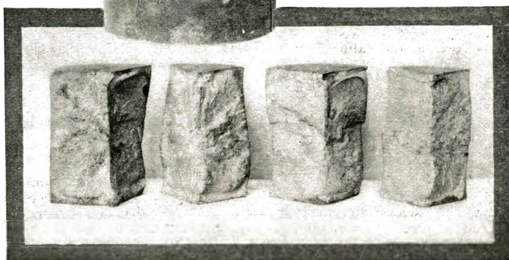
This Cylindrical Piece of Steel Burst at an Unexpected Moment and Nearly Killed a Tool-maker in the Great General Electric Works, Who Was Totally Unprepared for any Such Action as Here Occurred. The Photo Shows the Four Almost Equal Segments Into Which the Steel Cylinder Cracked, This Effect Being Attributed by Experts, to the Fact That Severe Internal Strains Were Set Up When the Steel Was Suddenly Cooled, and That This Resulted in the Sudden Bursting of the Solid Steel Piece.
