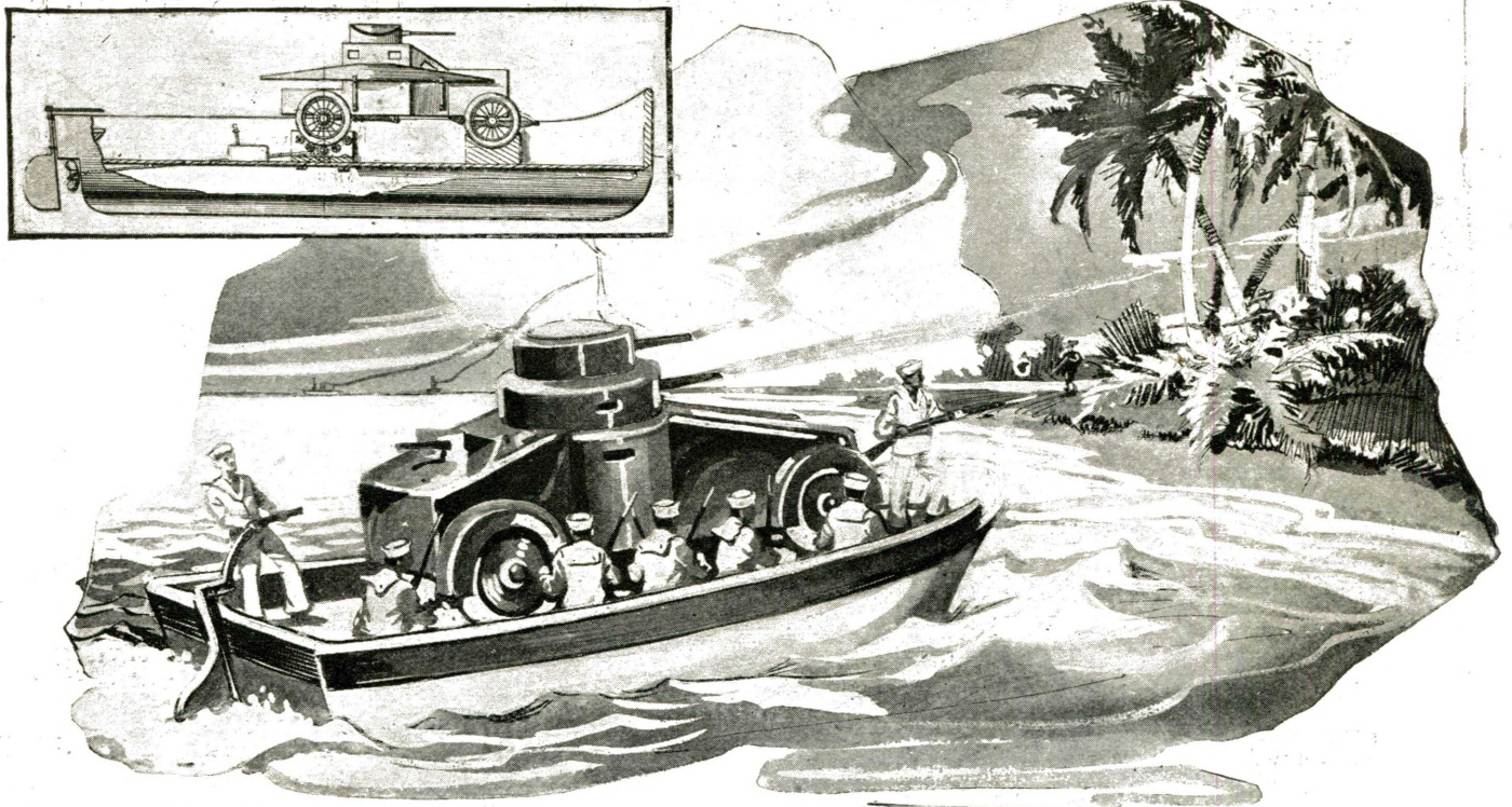
A Recently Patented Idea Which Will Find Extensive Adaptation in Future Warfare Maneuvers, Especially in Landing Troops or Marines As Here Shown. The Armored Motor-Car Is Caused to Propel the Landing Boat By Placing the Hind Wheels On a Series of Friction Rollers, Suitably Geared to the Propeller Shaft in the Manner Indicated in the Diagram at the Top of the Illustration. The Guns of the Armored Motor-Car Can Be Used While the Boat Is Moving, When Desired. The Front Wheels of the Motor-Car Rest in Grooved Chocking Blocks.
